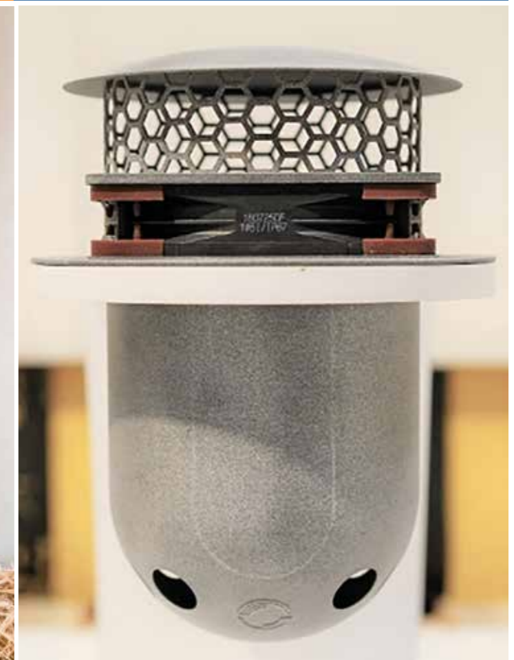
Klimasimulation vet.smart.iglustar
